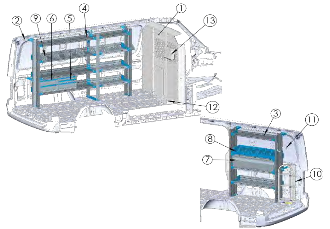
HVAC Essentials Package, Mercedes Sprinter Standard Roof 144", HVAC-SPSR144B
