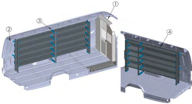
Base Shelving Package, Sprinter High Roof 170"X - BASE-SP-HR170X
