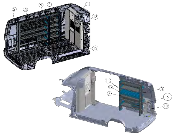
HVAC Essentials Package, Mercedes Sprinter High Roof 144", HVAC-SPHR144B
