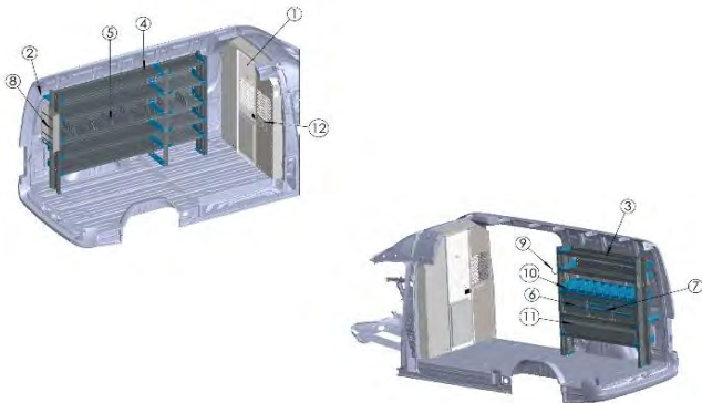
Electrical Essentials Package, Mercedes Sprinter High Roof 144", ELE-SPHR144B
