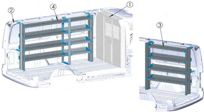
General Service Package, Mercedes Sprinter Standard Roof 144", GEN-SPSR144B
