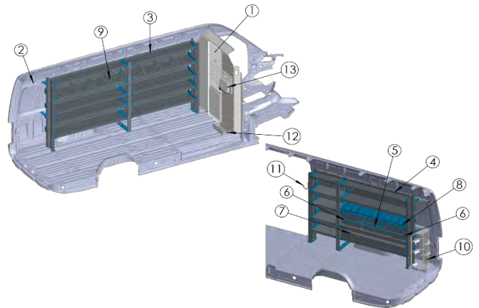
HVAC Essentials Package, Mercedes Sprinter High Roof 170", HVAC-SPHR170B
