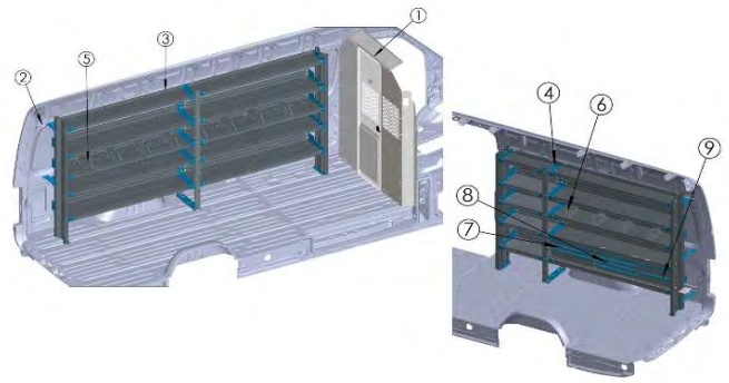
Bin Shelving Package, Sprinter High Roof 170" - BIN-SP-HR170
