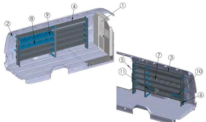
Plumbing Essentials Package, Mercedes Sprinter High Roof 170" Extended, PLUM-SPHR170XB
