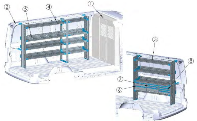
Bin Shelving Package, Sprinter Low Roof 144" - BIN-SP-SR144
