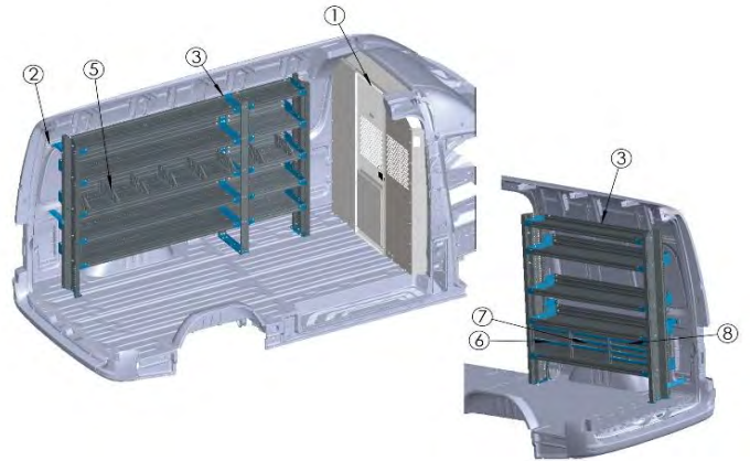
Bin Shelving Package, Sprinter High Roof 144 - BIN-SP-HR144
