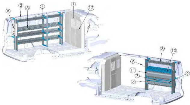
Electrical Essentials Package, Mercedes Sprinter Standard Roof 144", ELE-SPSR144B
