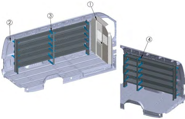
Base Shelving Package, Sprinter High Roof 170" - BASE-SP-HR170
