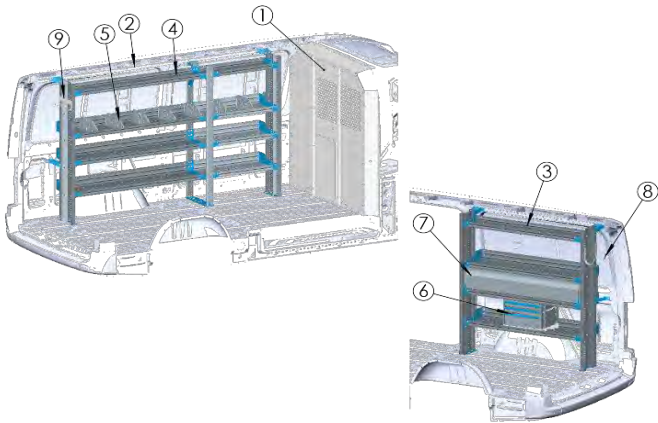
Electrical Essentials Package, Mercedes Sprinter Standard Roof 144", ELE-SPSR144B
